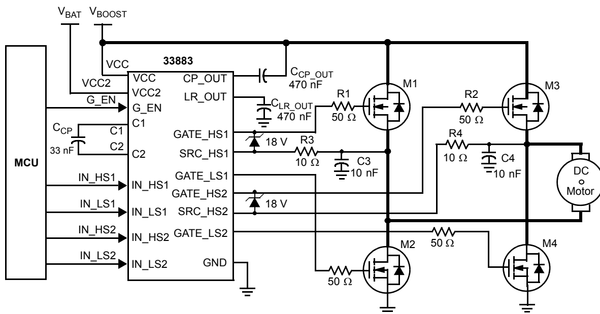
Figure 14. Application Schematic with External Protection Circuit
