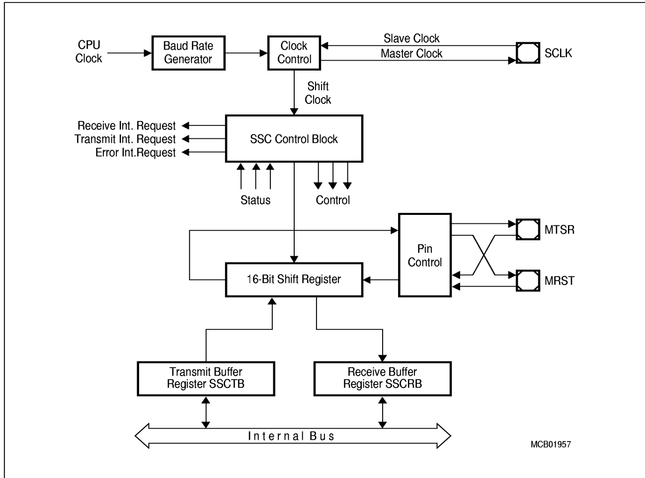
Figure 61 Synchronous Serial Channel SSC Block Diagram
