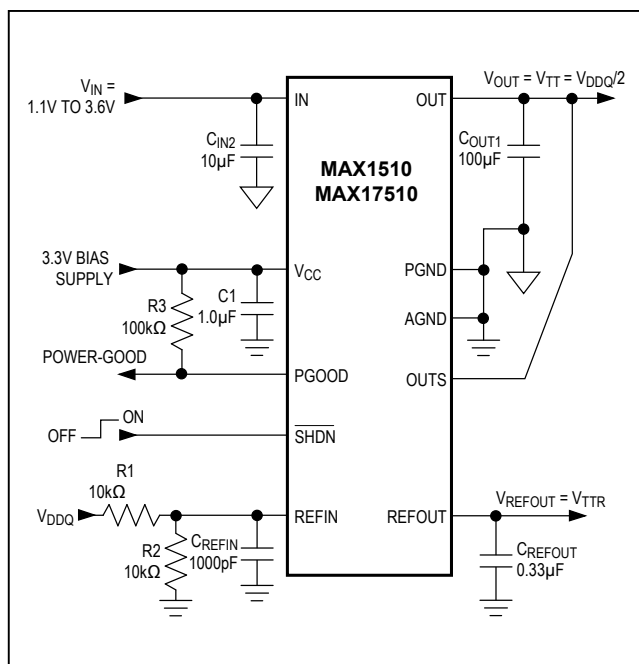
Figure 1. Standard Application Circuit
