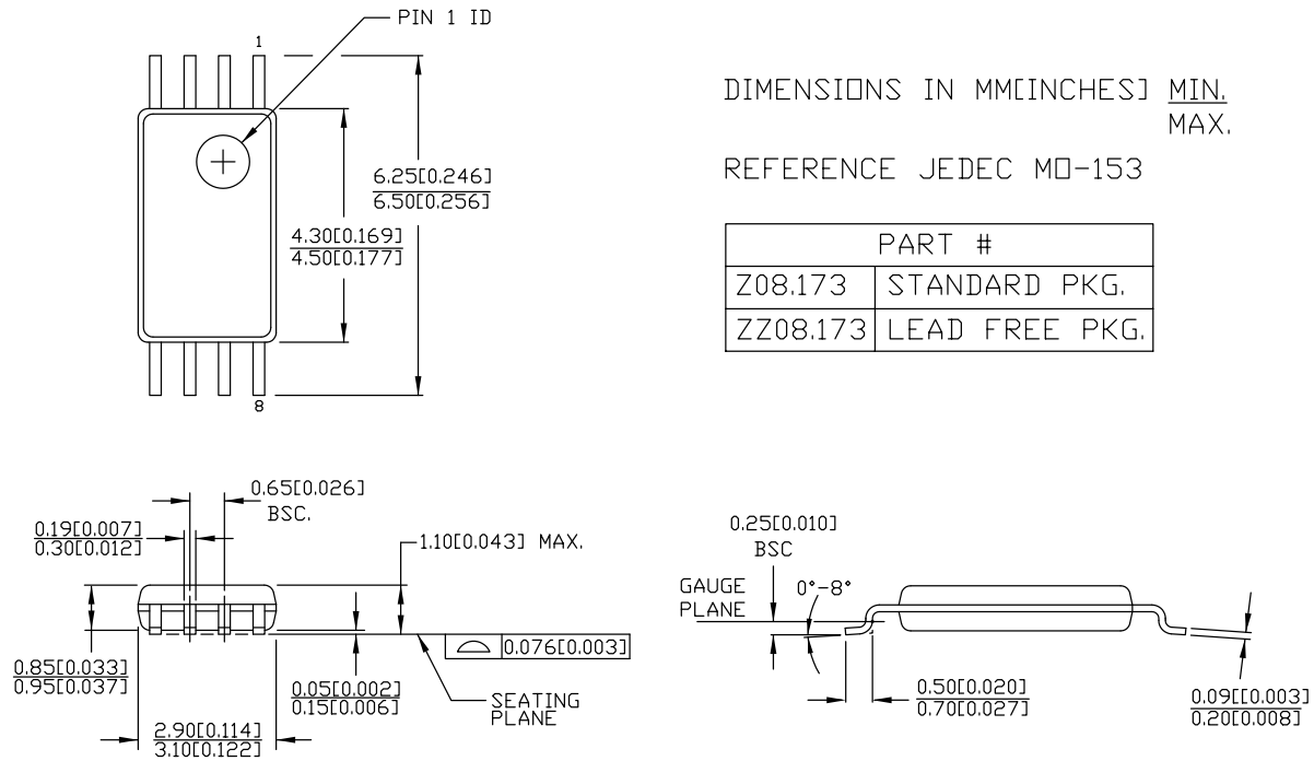
Figure 7. 8-pin TSSOP (4.40 mm Body) Z08.173/ZZ08.173 Package Outline, 51-85093
