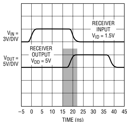
Propagation Delay Guaranteed to Fall Within Shaded Area ( \pm 3.5ns )
