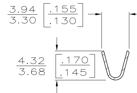
SECT B-B
