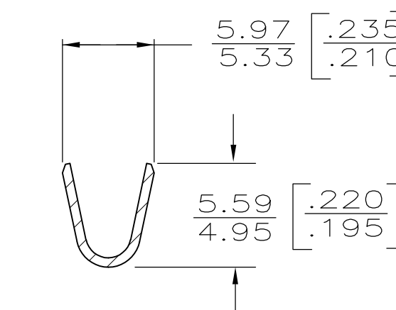
SECT C-C
