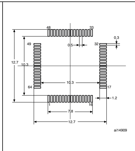
Figure 43. Recommended footprint
