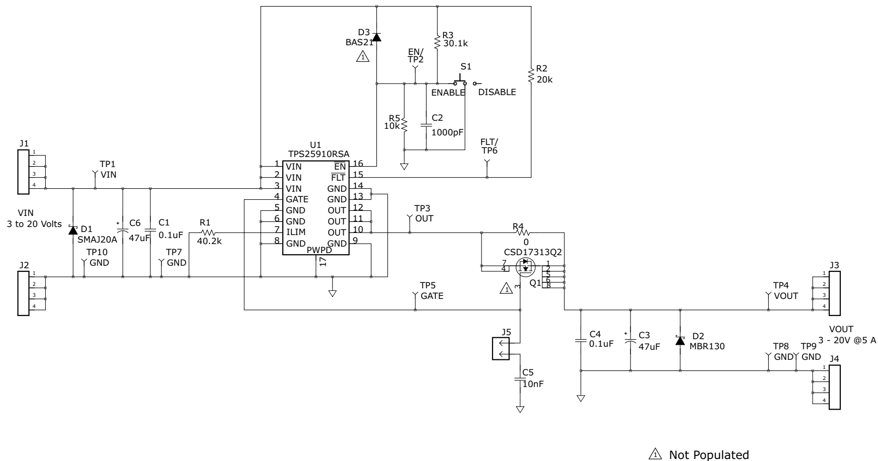
Figure 1. TPS25910EVM-088 Schematic
