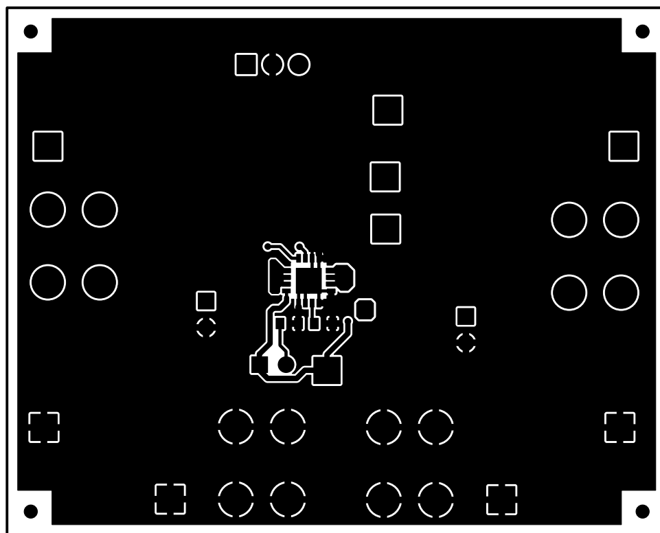
Figure 4. Top-Side Routing
