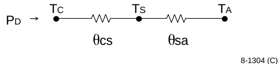
Figure 33. Resistance from Case-to-Sink and Sink-to-Ambient
