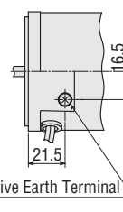
Detail Drawing of Protective Earth Terminal
