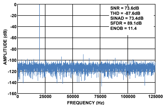
FIGURE 17. SINGLE-TONE FFT
