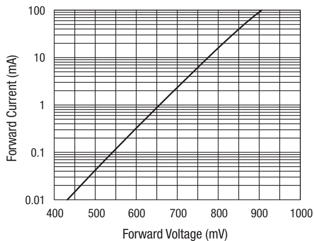
Figure 3. DC Characteristic
