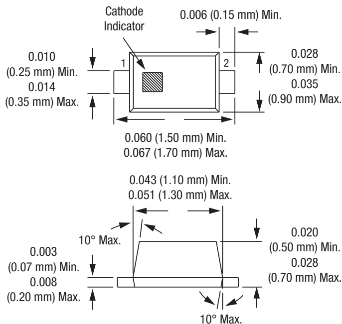
Figure 8. SC-79 Package Dimension Drawing
