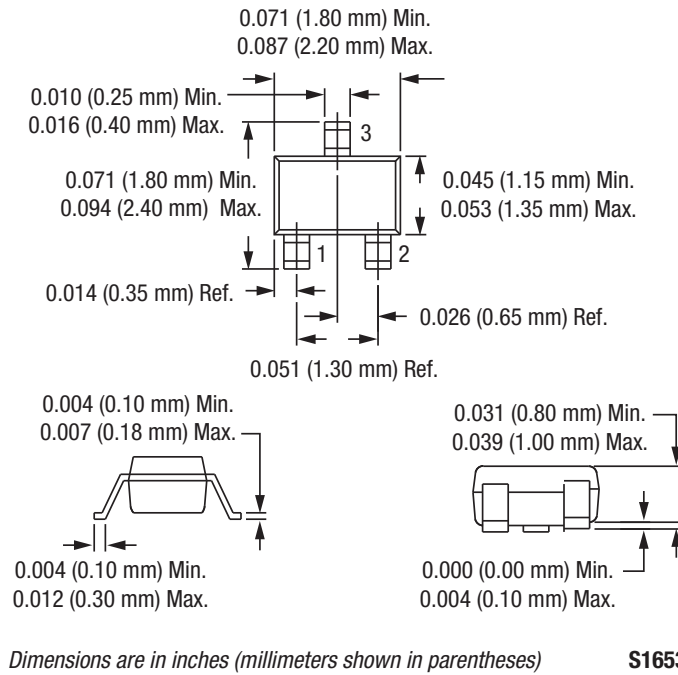
Figure 6. SC-70 Package Dimension Drawing
