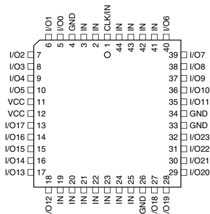
Figure 2-2. PLCC
