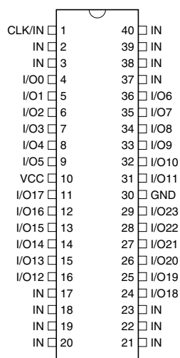
Figure 2-1. DIP
