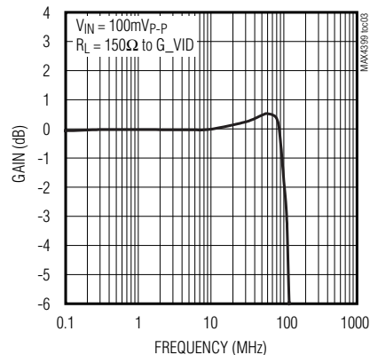
RGB VIDEO SMALL-SIGNAL BANDWIDTH vs. FREQUENCY
