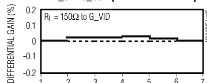
RF_CVBS_OUT (WITH TRAP FILTER)
