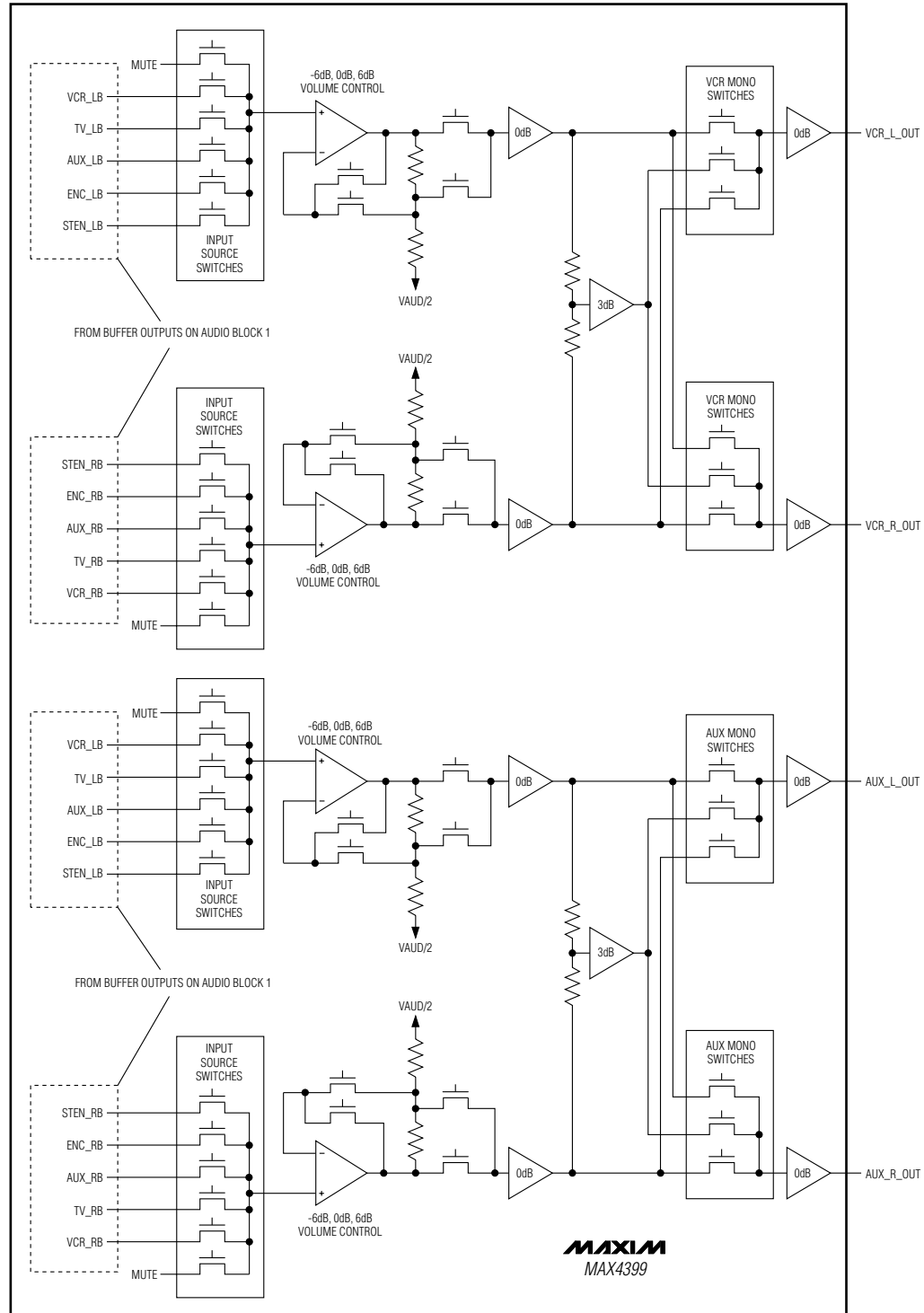
Figure 4. Audio Functional Diagram (AUDIO BLOCK2)
