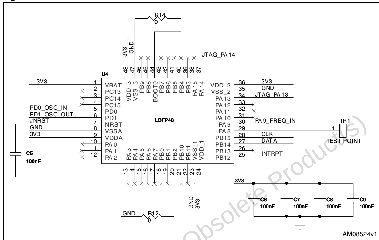
Figure 2. Schematic 2 of 5
