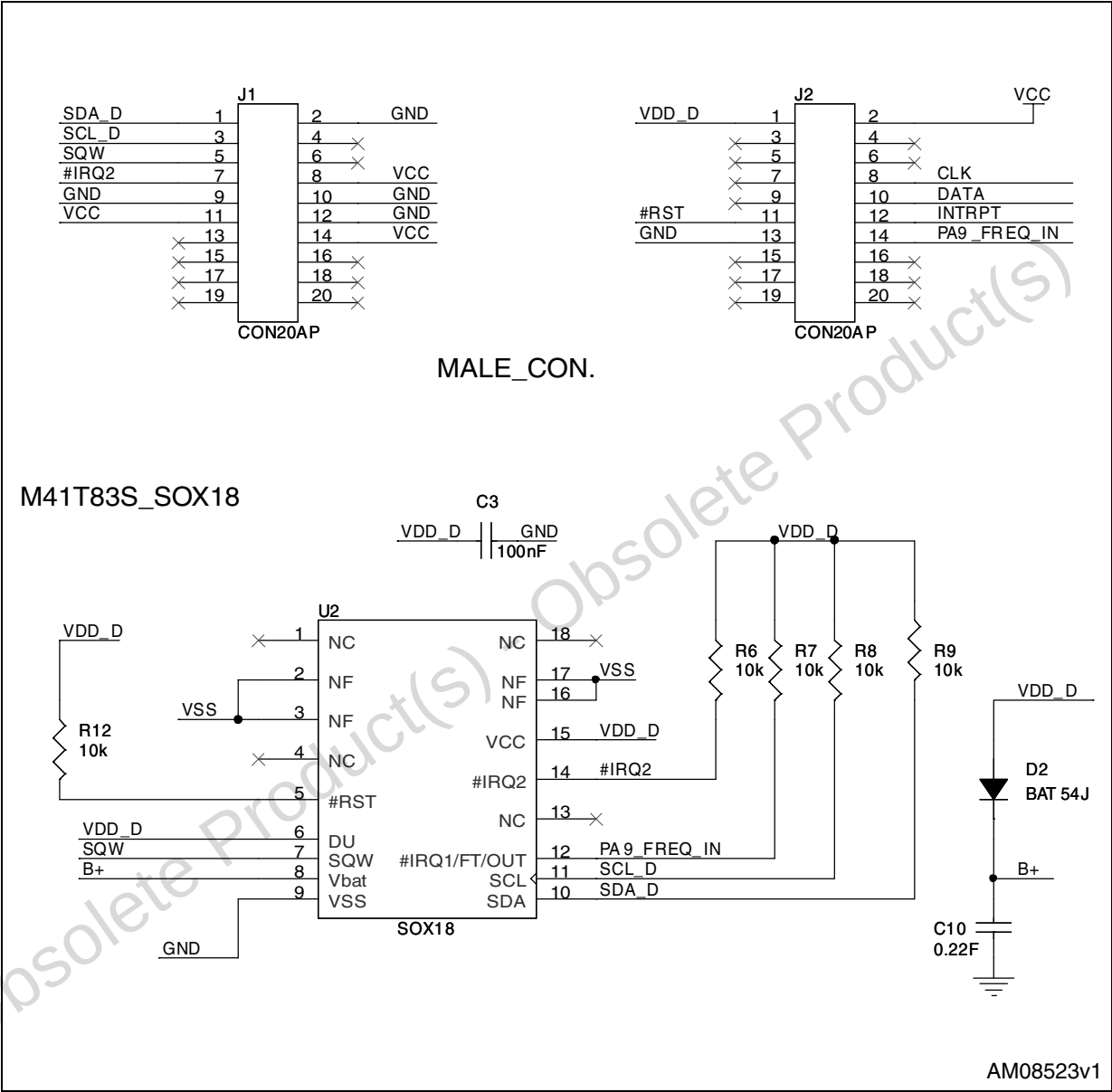
Figure 1. Schematic 1 of 5
