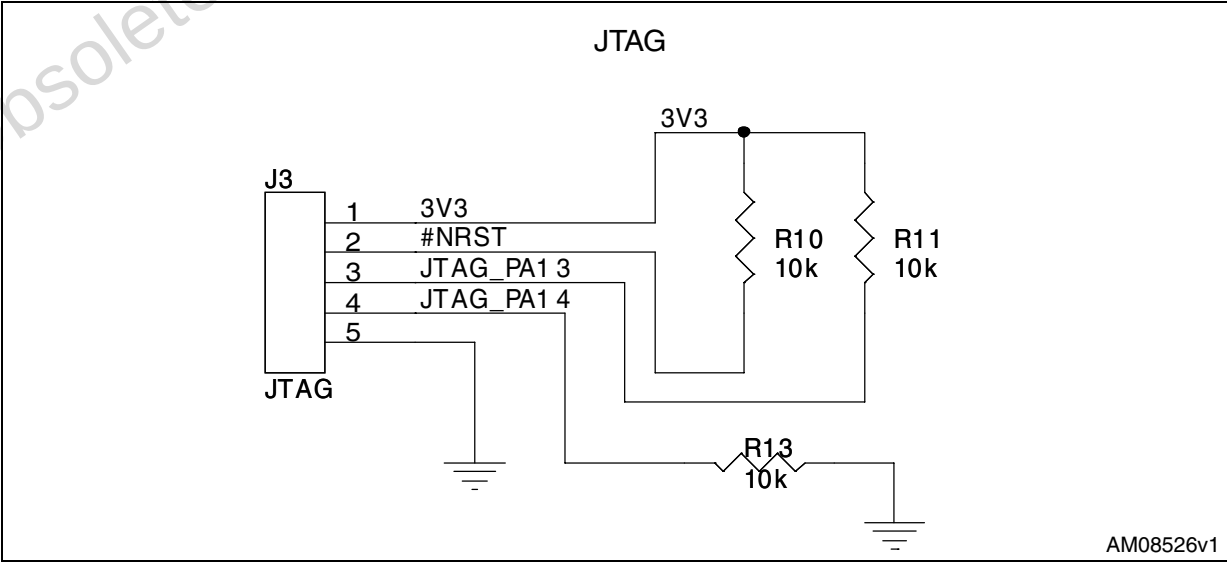
Figure 4. Schematic 4 of 5 (JTAG)
