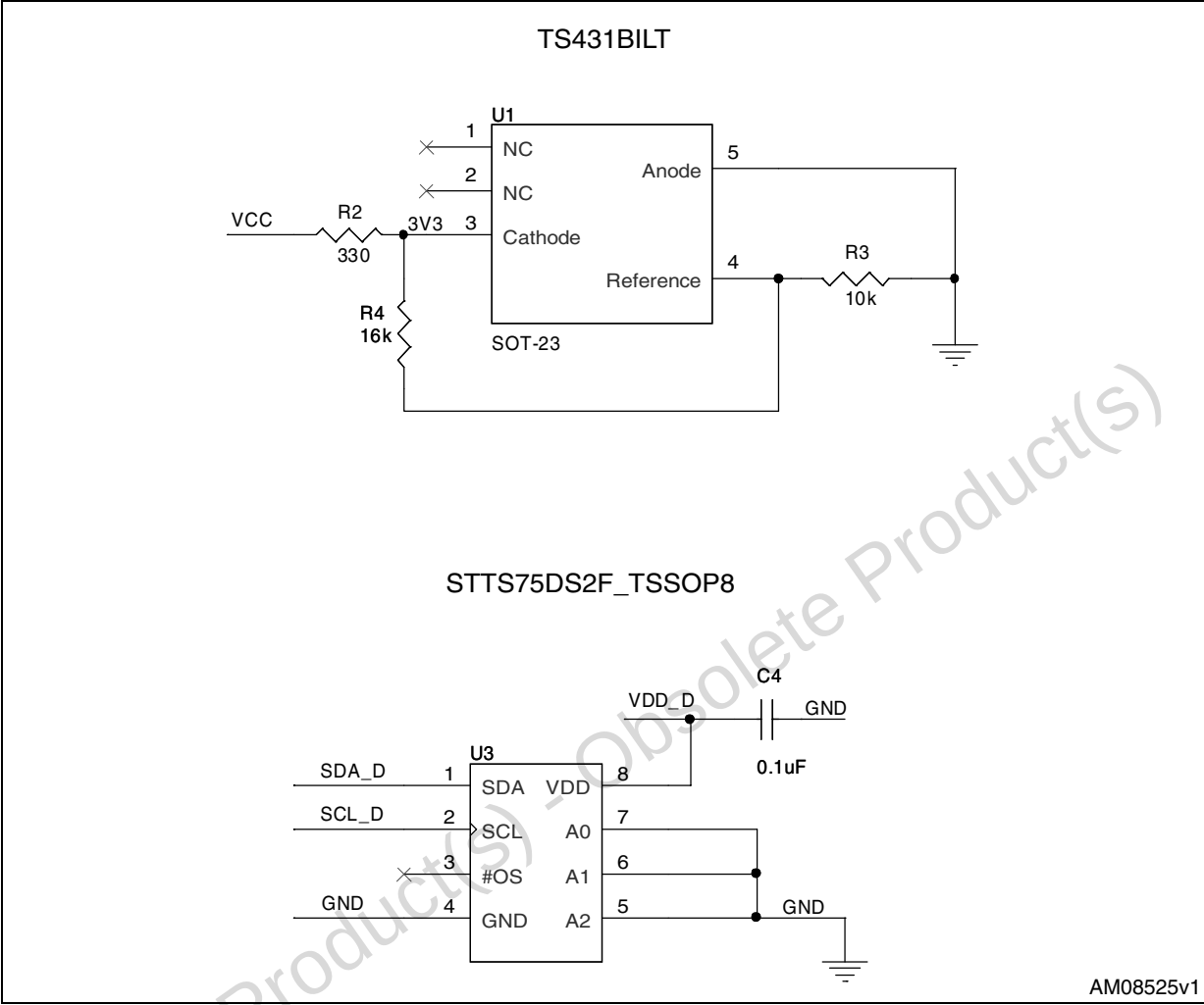
Figure 3. Schematic 3 of 5
