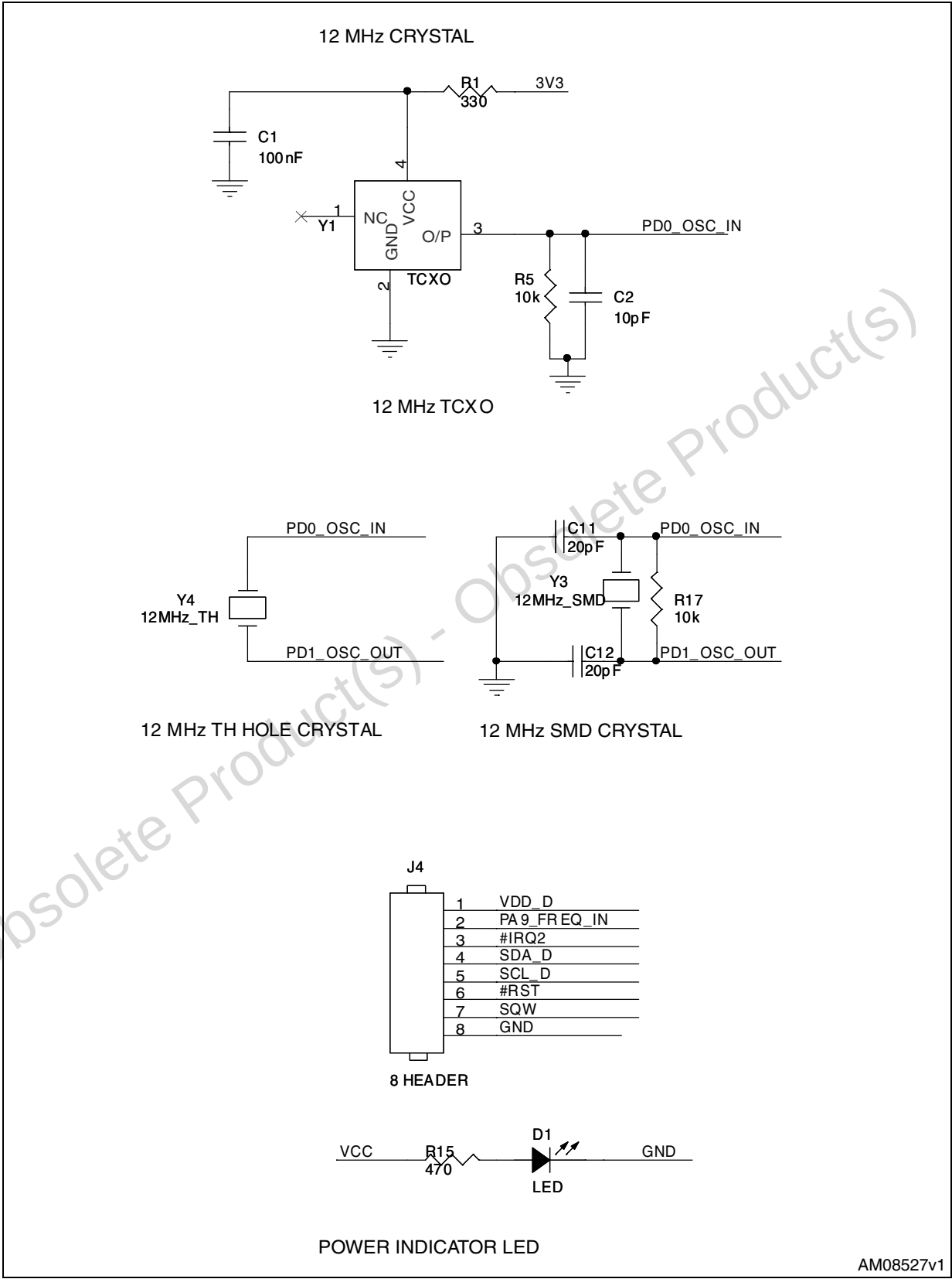
Figure 5. Schematic 5 of 5
