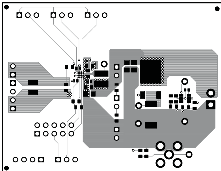
Figure 13. Top Layer
