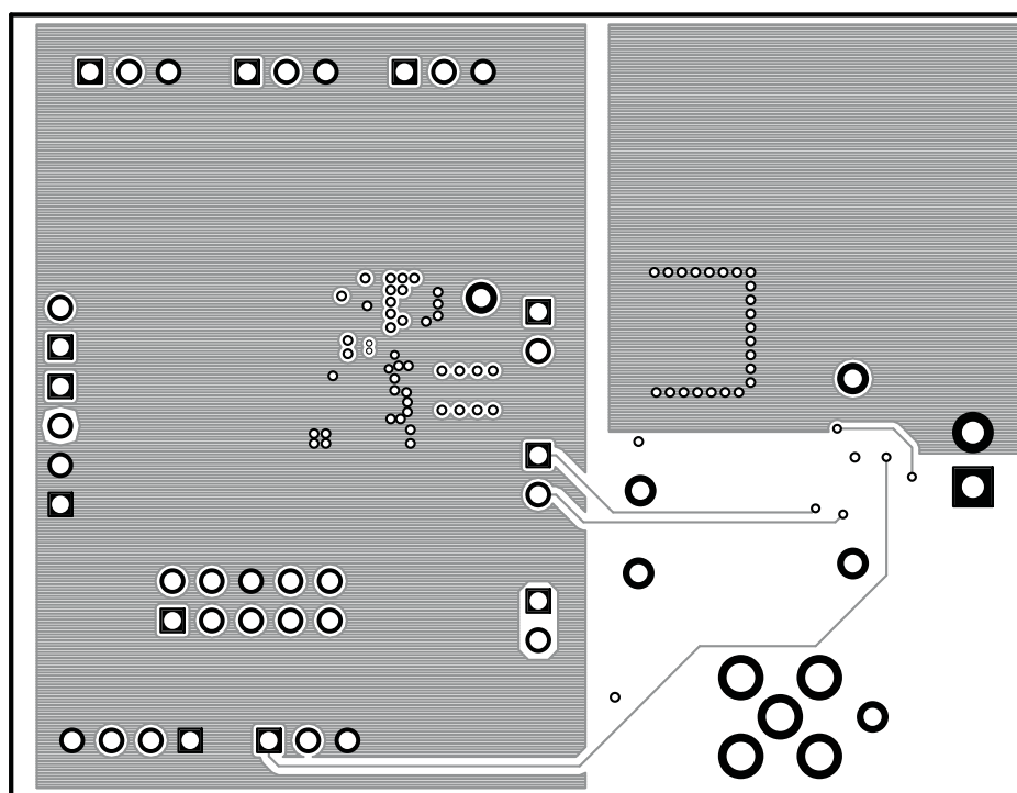
Figure 14. Layer 2
