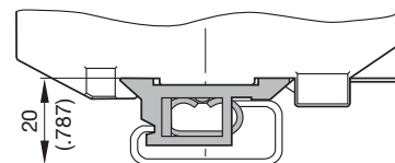
*Adapter foot – dimensions in mm (in.)
