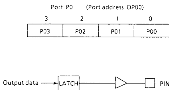
Figure1-1. Port P0
