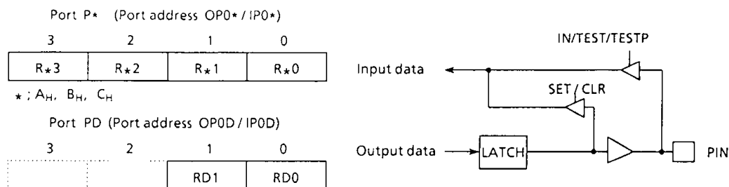
Figure1-3. Ports RA through RD
