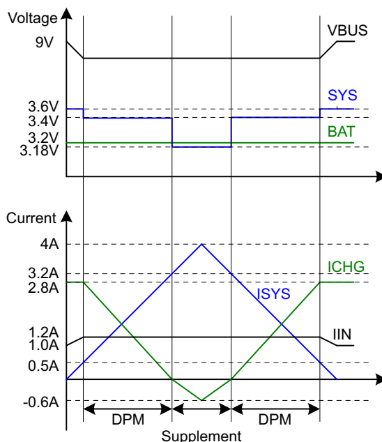
Figure 27. DPM Response
