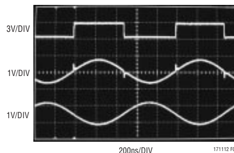
Figure 8. Oscillator Waveforms with V_S = 3V . Top is Comparator Output. Middle is Xtal Feedback to Pin 2 at LT1713 (Note the Glitches). Bottom is Buffered, Inverted and Bandpass Filtered with a Q = 5 by LT1806
