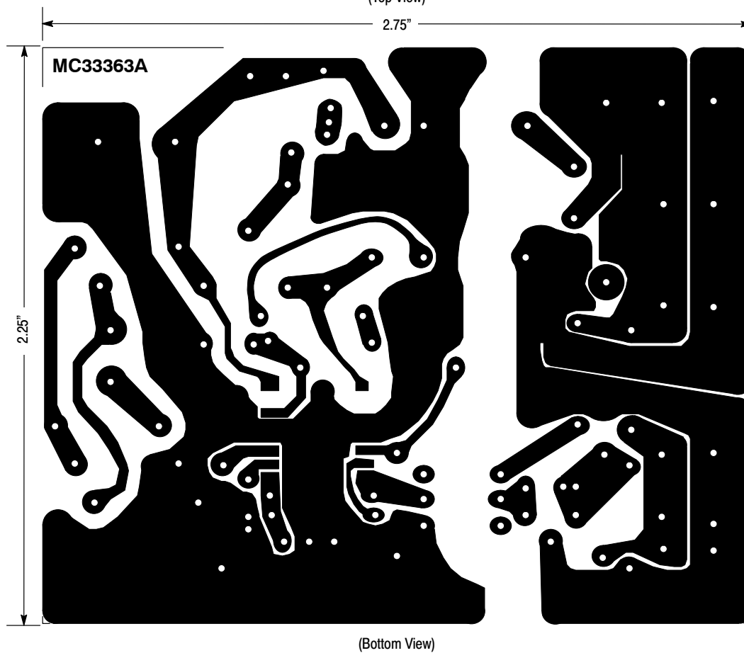
Figure 23. Printed Circuit Board and Component Layout (Circuit of Figure 22)
