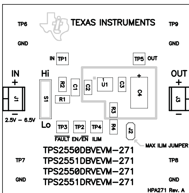
Figure 5. EVM Top Assembly
