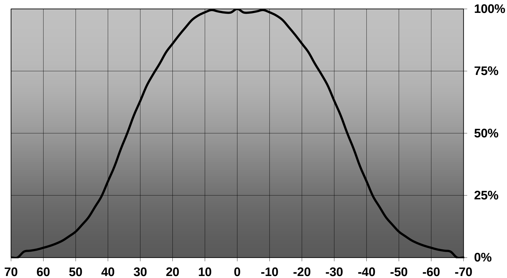
Relative intensity of Laura-WW-Pin-XP-G
