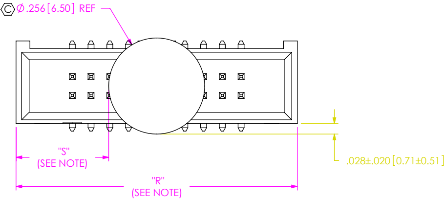
FIG 4 (SHF-110-01-X-D-SM-K SHOWN) (SAME AS FIG 1, DIFFERENT AS SHOWN)
