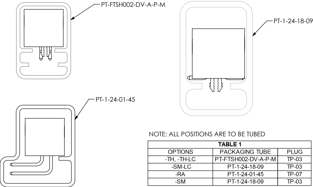
FIG 4 (SHF-110-01-X-D-SM-K SHOWN) (SAME AS FIG 1, DIFFERENT AS SHOWN)
