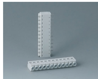
B6603111 Terminal block, block 5.0 mm PA 68 (UL 94 V-0)
