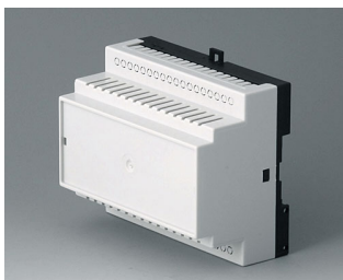
B6504119 RAILTEC B, 6 modules, Vers. V PC (UL 94 V-0) light gray RAL 7035 4.13"x3.39"x2.32"
