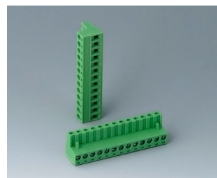
B6605223 Plug header, block 5.08 mm PA 6 (UL 94 V-0)
