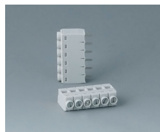
B6607111 Terminal block, block 5.0 mm PA 68 (UL 94 V-0)
