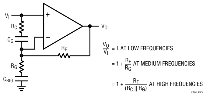
Figure 12. Combination Compensation
