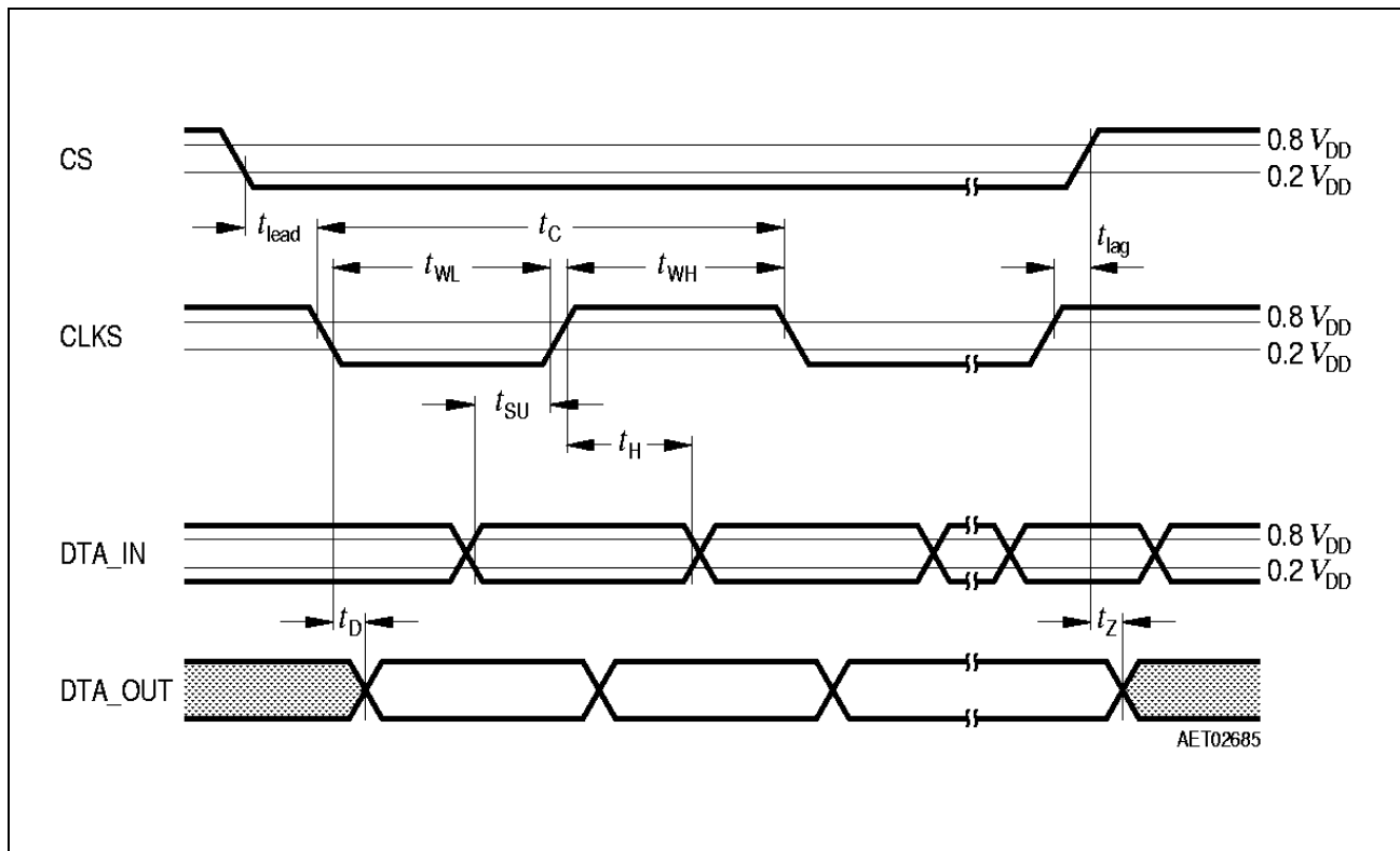
Figure 4 Serial Peripheral Interface: Timing Diagram
