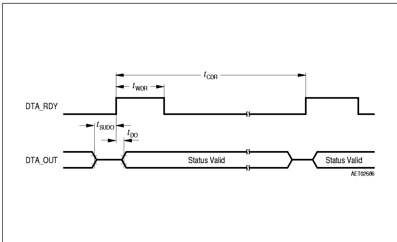
Figure 5 DTA_RDY Timing Diagram
