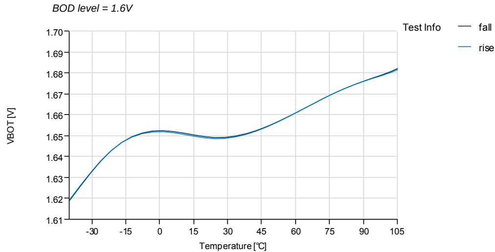
Figure 37-60.BOD thresholds vs. temperature.
