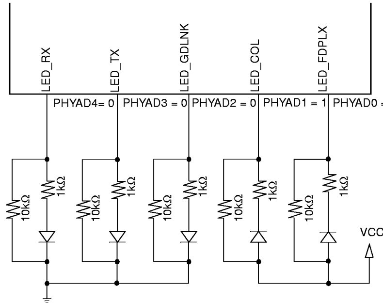
Figure 2. PHYAD Strapping and LED Loading Example
