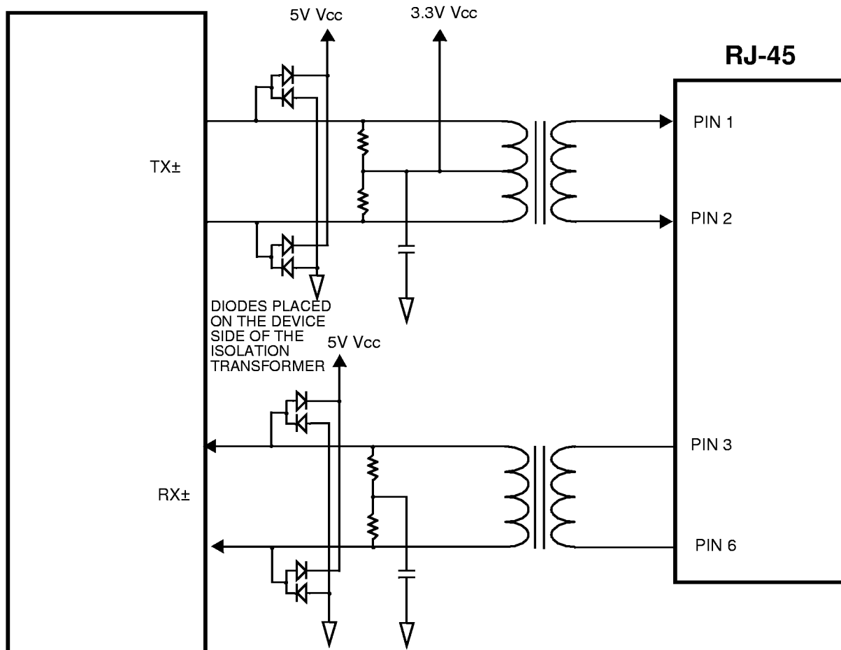
Figure 10. Typical DP83849A Network Interface with additional ESD protection
