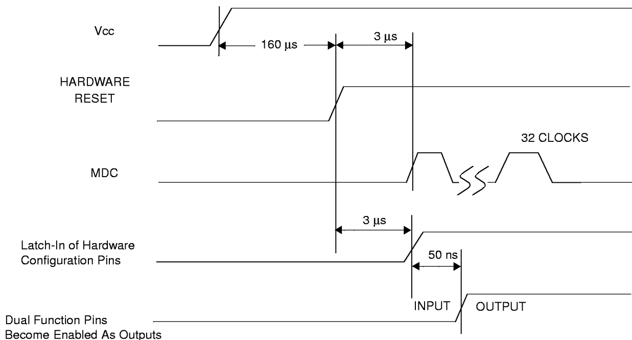
Figure 11. Power-on Reset Examples
