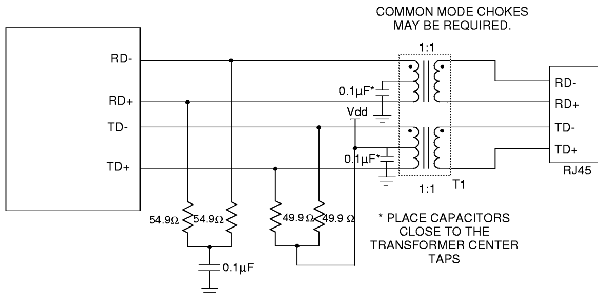
Figure 9. 10/100 Mb Interface
