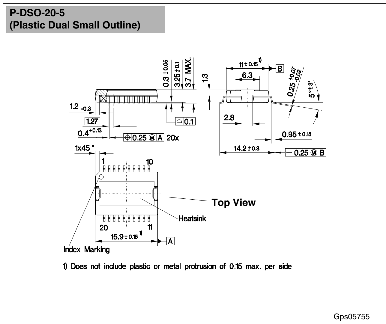
Figure 97 SLIC-S/-S2, SLIC-E/-E2, SLIC-P (PEB 426x)
