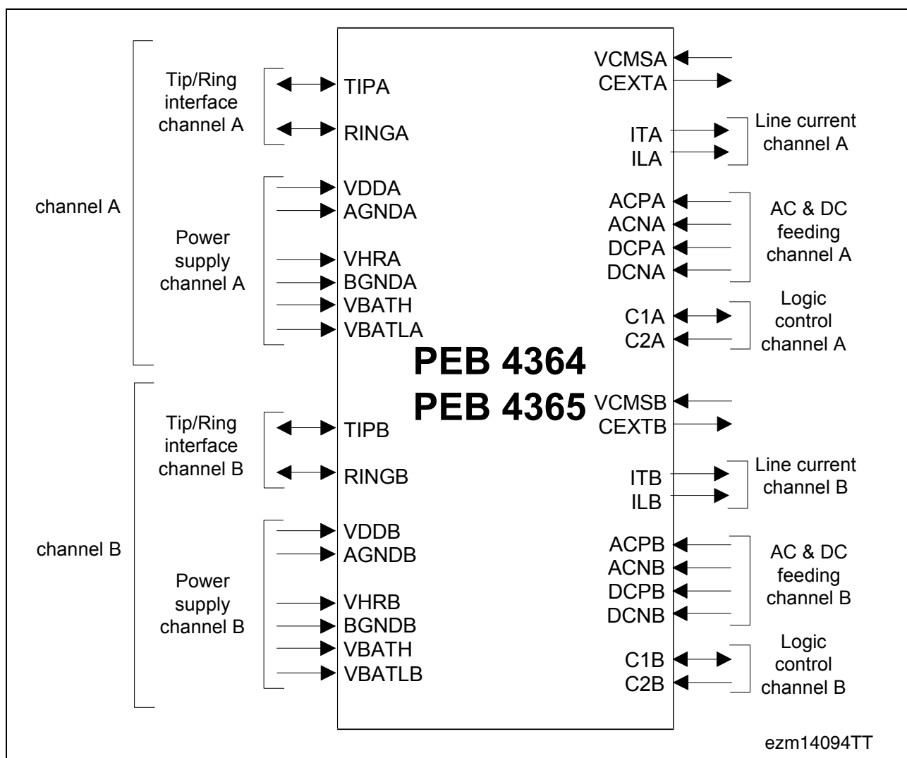
Figure 6 Logic Symbol: TSLIC-S/TSLIC-E
