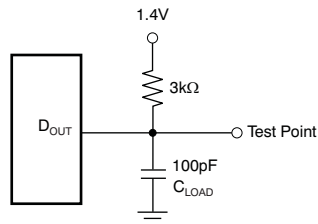
Load Circuit for t_{\text{dD}} , t_{\text{r}} , and t_{\text{f}}
