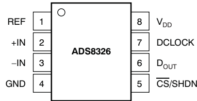
DRB PACKAGE SON-8 (TOP VIEW)
