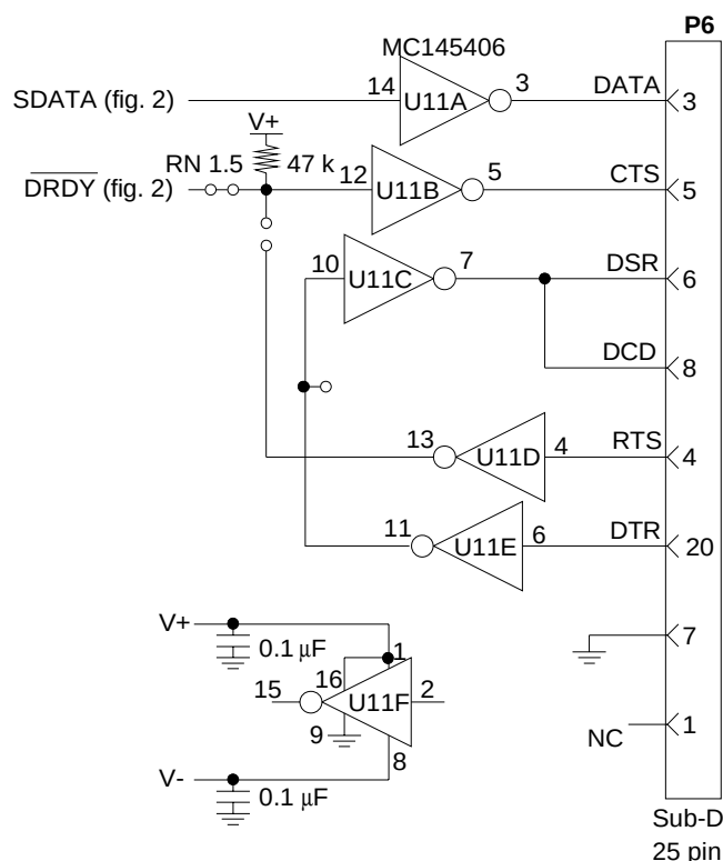
Figure 4. RS-232 Port
