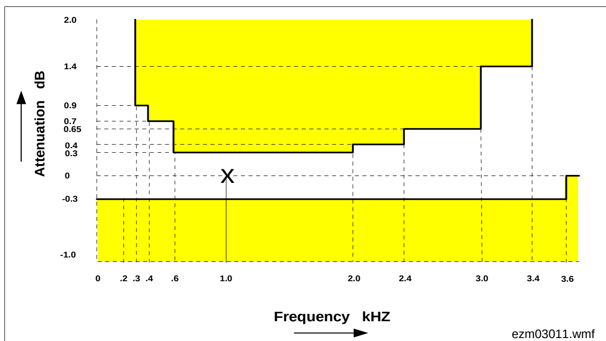
Figure 35 Frequency Response Receive
