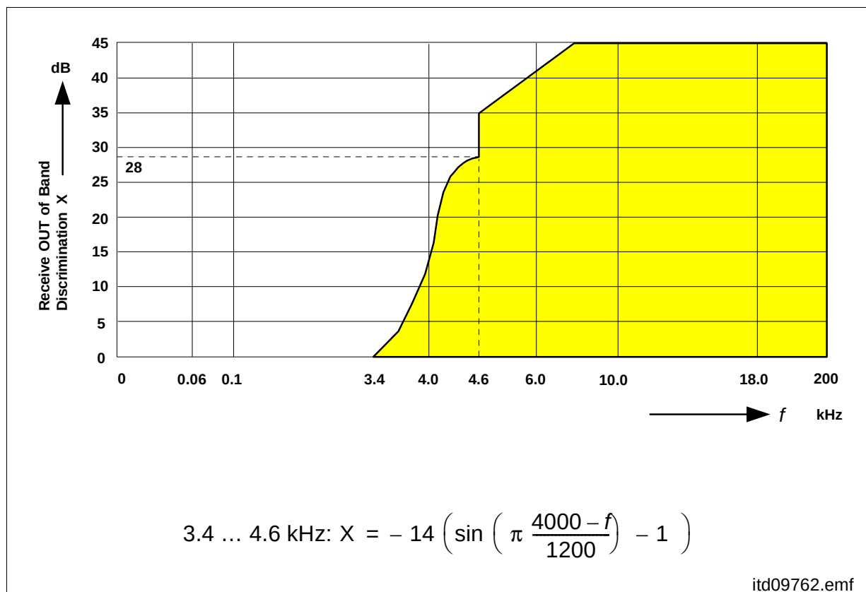
Figure 41 Out-of-Band Signals at Analog Output (Receive)
