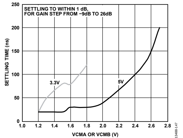
Figure 46. Maximum Gain Transition Settling Time vs. Output Common-Mode Voltage (VCMA or VCMB)
