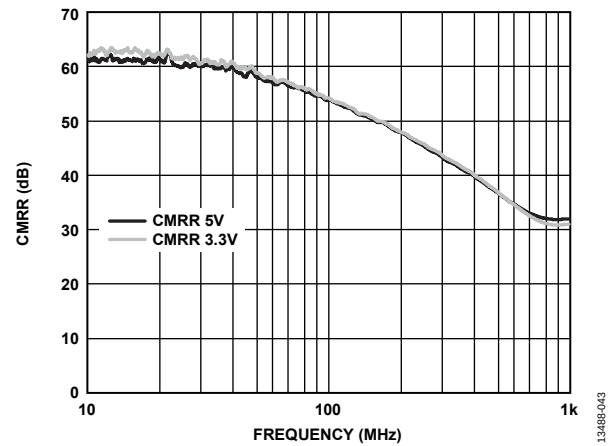
Figure 45. CMRR vs. Frequency at Maximum Gain
