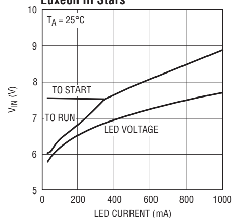
Minimum Input Voltage, Two Series Connected White Luxeon III Stars
