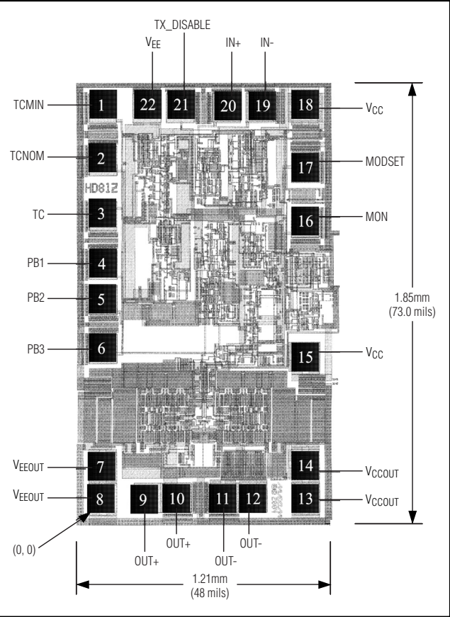
Chip Topography
