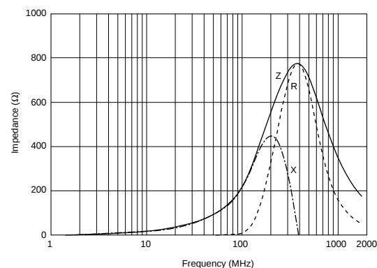
BLM18BB221SH1
