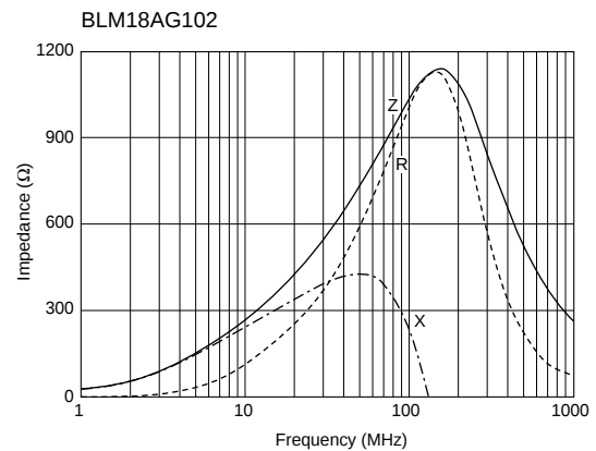
[Example of impedance frequency characteristics of inductor type EMIFIL®]
