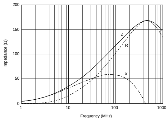
BLM18AG121SH1
