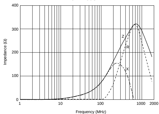
BLM18BB750SH1
