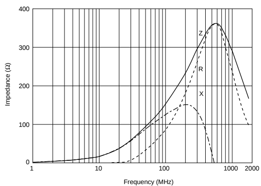
BLM18BD151SH1
