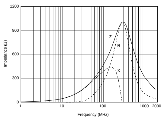
BLM18BD471SH1
