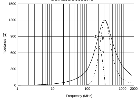
BLM18BB331SH1
