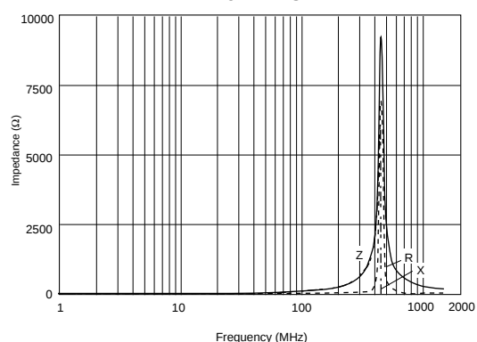
BLM18BA121SH1
