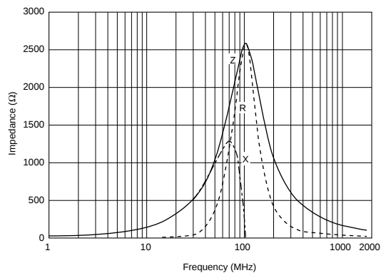
BLM18BD252SH1
