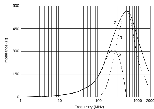
BLM18BB151SH1
