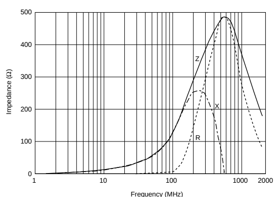
BLM18BB121SH1
