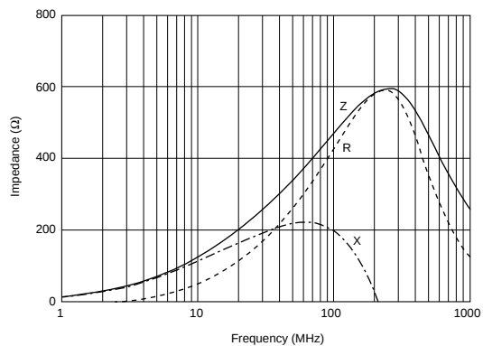
BLM18AG471SH1
