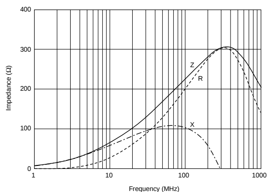
BLM18AG221SH1
