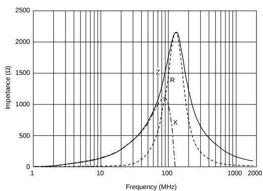
BLM18BD182SH1
