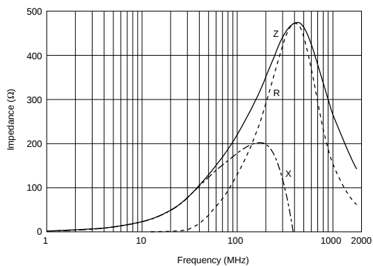
BLM18BD221SH1
