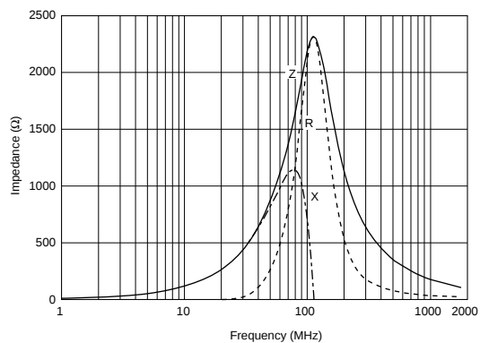
BLM18BD222SH1
