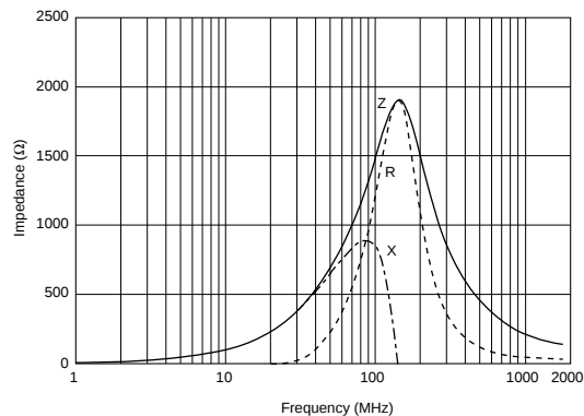
BLM18BD152SH1
