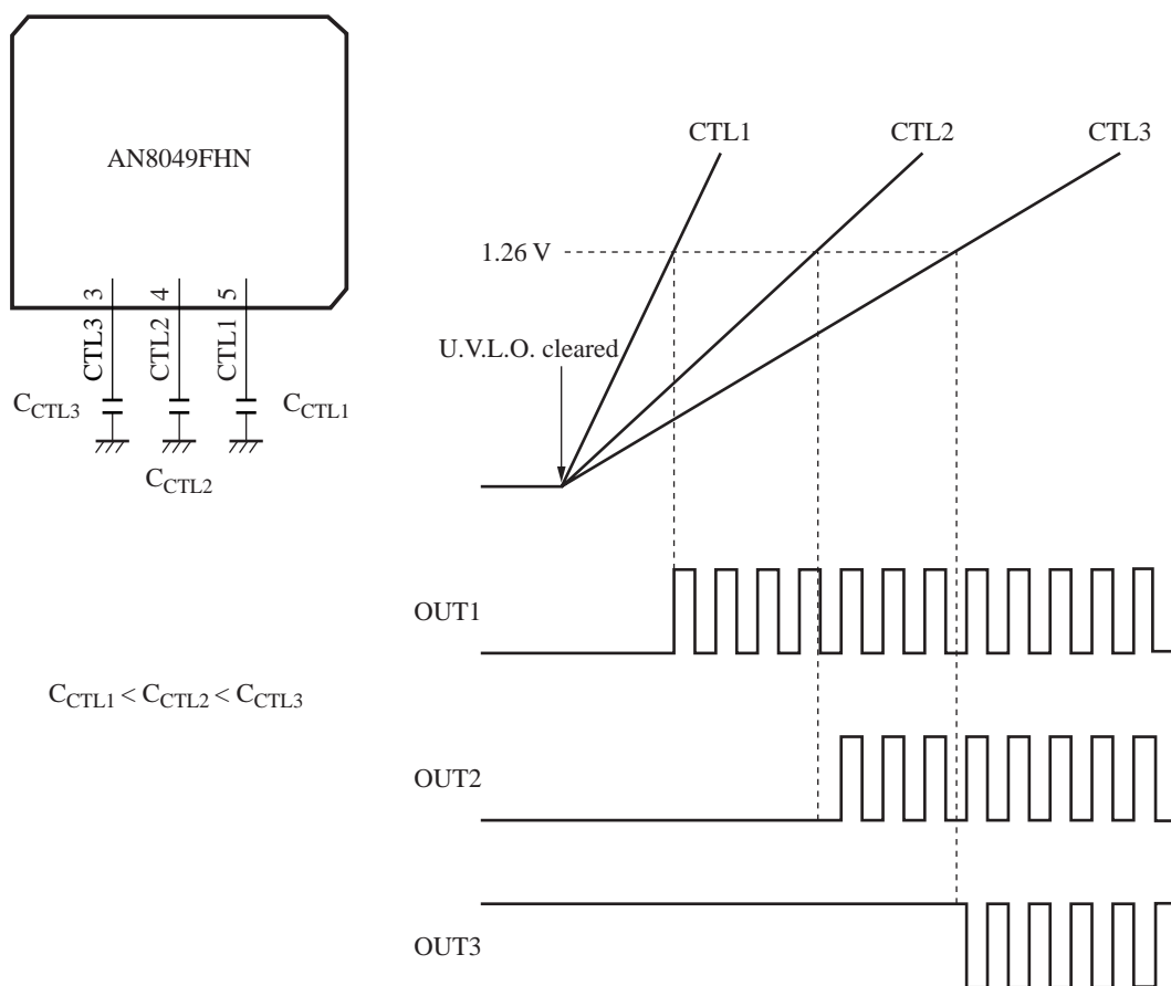
Figure 8. Sequential operation
