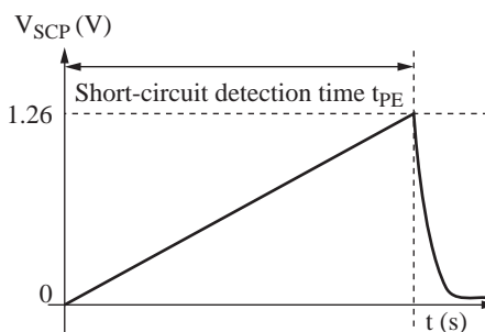
Figure 5. S.C.P. pin charging waveform
