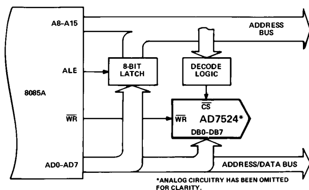
Figure 6. AD7524/8085A Interface
