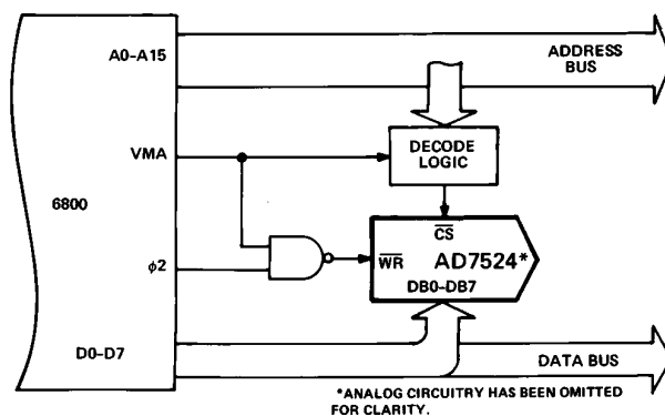
Figure 7. AD7524/MC6800 Interface
