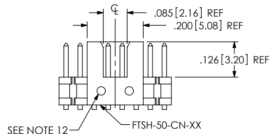
FIG 3 -A OPTION (DIFFERENT AS SHOWN, OTHERWISE SAME AS FIG 1) (6 POSITION MINIMUM FOR STAKED ALIGNMENT PINS) (3 POSITION MINIMUM FOR MOLDED ALIGNMENT PINS)
