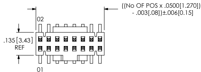
FIG 2 -K OPTION (LEAD STYLE -01 ONLY) (DIFFERENT AS SHOWN, OTHERWISE SAME AS FIG 1) (POSITION 13, 17, 20 & 25 AVAILABLE WITH -EJ OPTION)
