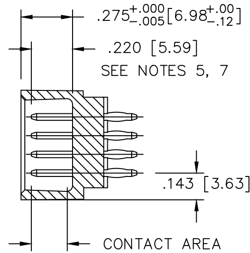
SECTION X—X
