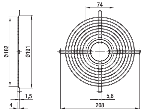
Guard grille for diagonal fan
