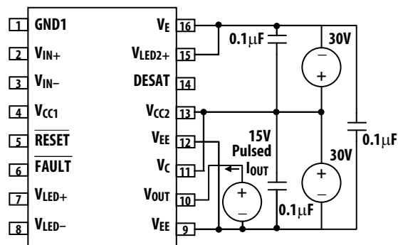
Figure 32. I_{OLO} pulsed test circuit.
