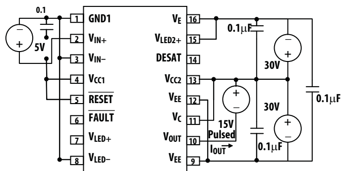
Figure 31. I_{OHP} pulsed test circuit.
