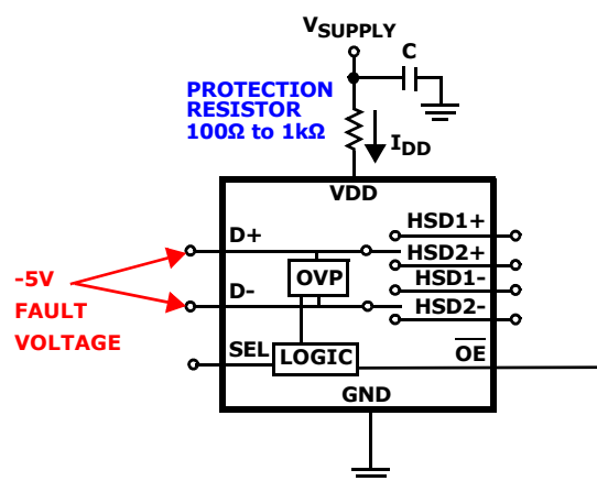
FIGURE 7. V_{DD} SERIES RESISTOR TO LIMIT I_{DD} CURRENT DURING NEGATIVE OVP AND FOR ENHANCED ESD AND LATCH-UP IMMUNITY
