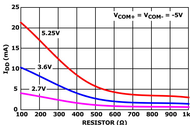
FIGURE 8. NEGATIVE OVP I_{DD} CURRENT vs RESISTOR VALUE vs V_{SUPPLY}
