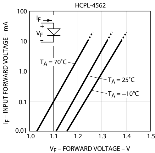
Figure 5 Input Current vs. Forward Voltage (HCPL-4562)
