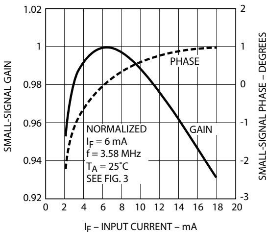
Figure 9 Small-Signal Response vs. Input Current (HCPL-4562)
