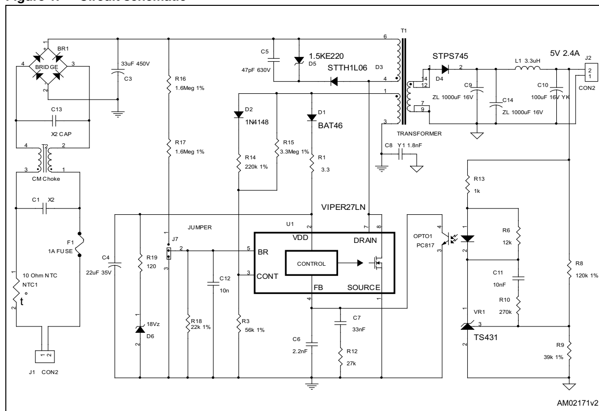
Figure 1. Circuit schematic
