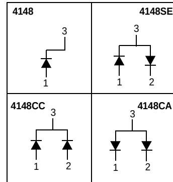
Connection Diagram
