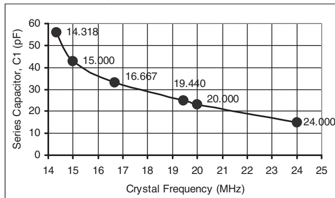
FIGURE 3B. Recommended tuning capacitance for various parallel resonant crystals.
