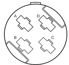
Tri-Start (MIL-DTL-38999, Series III) Connectors with MT Ferrule Inserts
