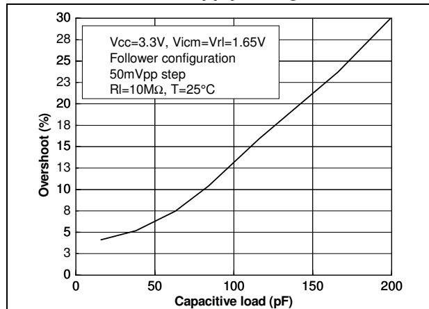
Figure 24. Overshoot vs. capacitive load at 3.3 V supply voltage
